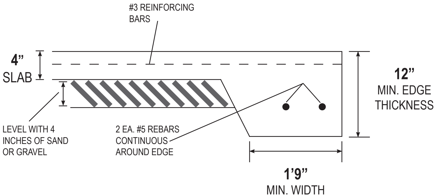
SECTION VIEW OF END OF SLAB
